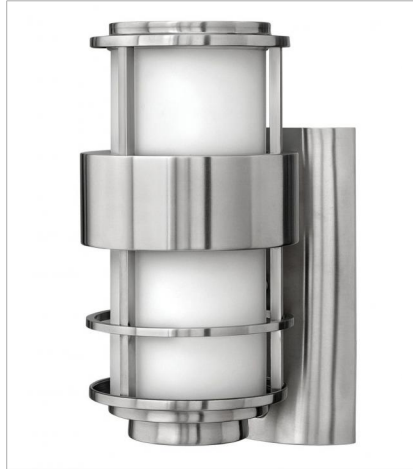
1900SS SMALL WALL MOUNT LANTERN 6" W, 12" H Socket 1-60w Med.
