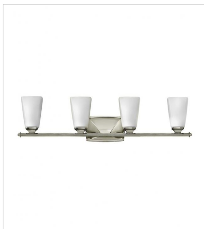
53014PN FOUR LIGHT VANITY 32" W, 8" H Socket 4-100w Incan. OR 4-17w LED Med.
